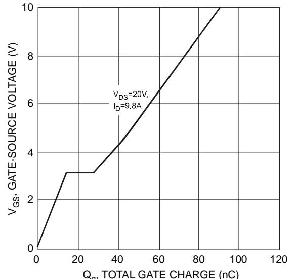
Fig. 10 Gate-Charge Characteristics
